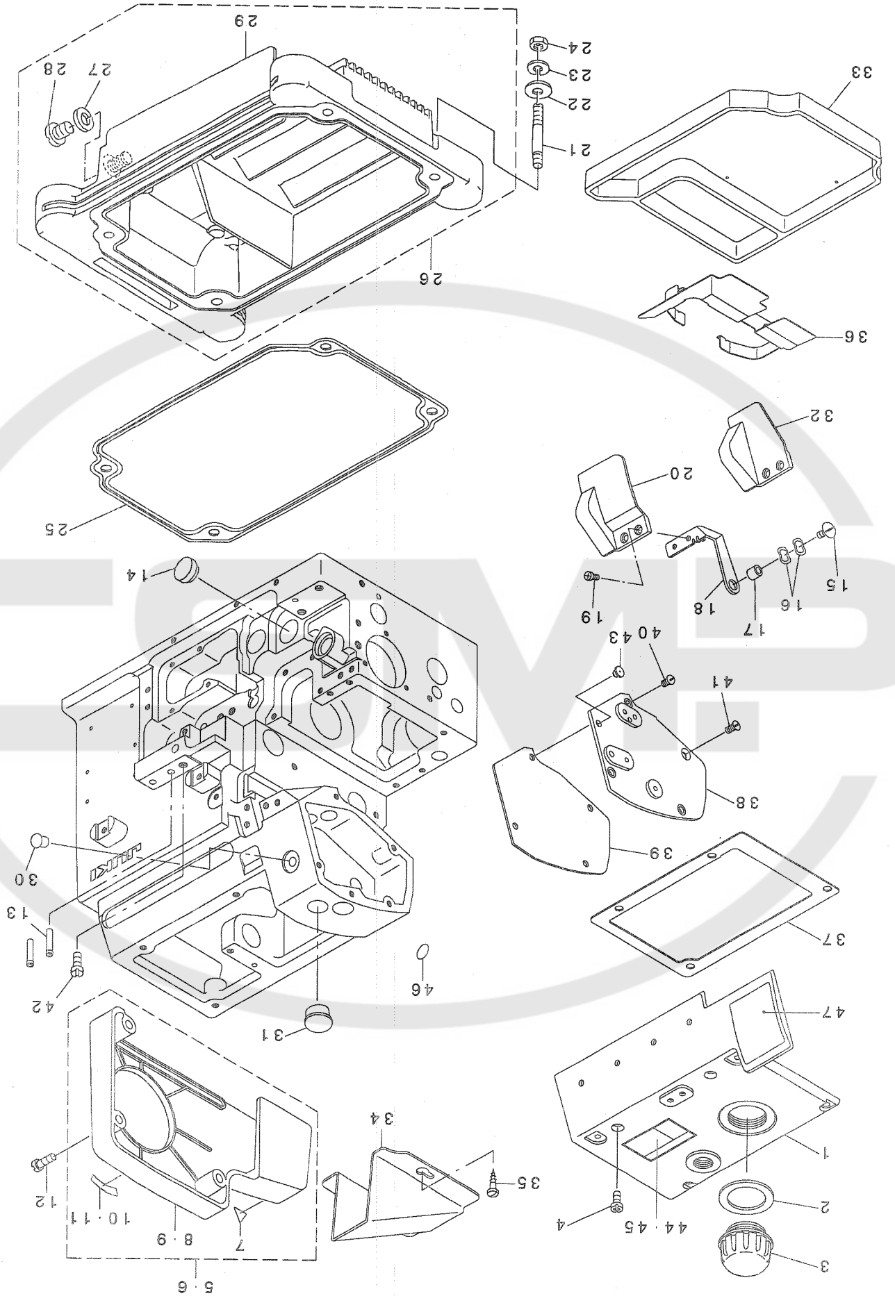
2. FRAME COMPONENTS(2) 71-△關係 (2)
